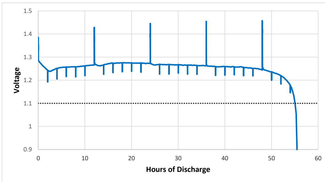
Typical IEC Standard Discharge Performance
